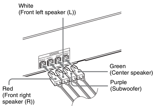
Rear panel of the unit
